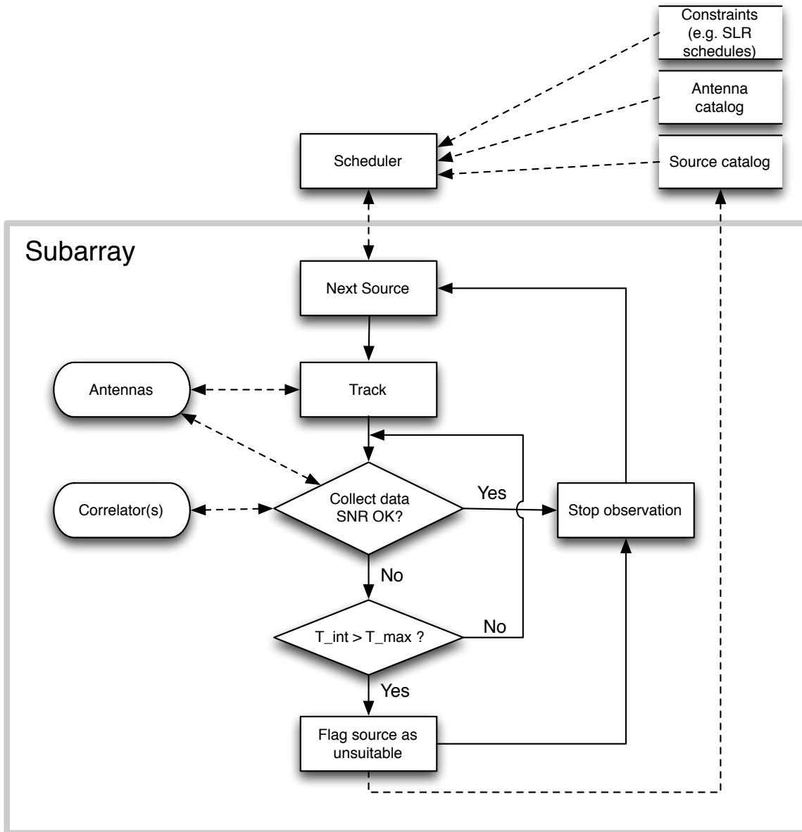
Figure 1: A flow chart describing the main observing cycle. Solid lines indicate flow while dashed lines indicate communication between elements.
