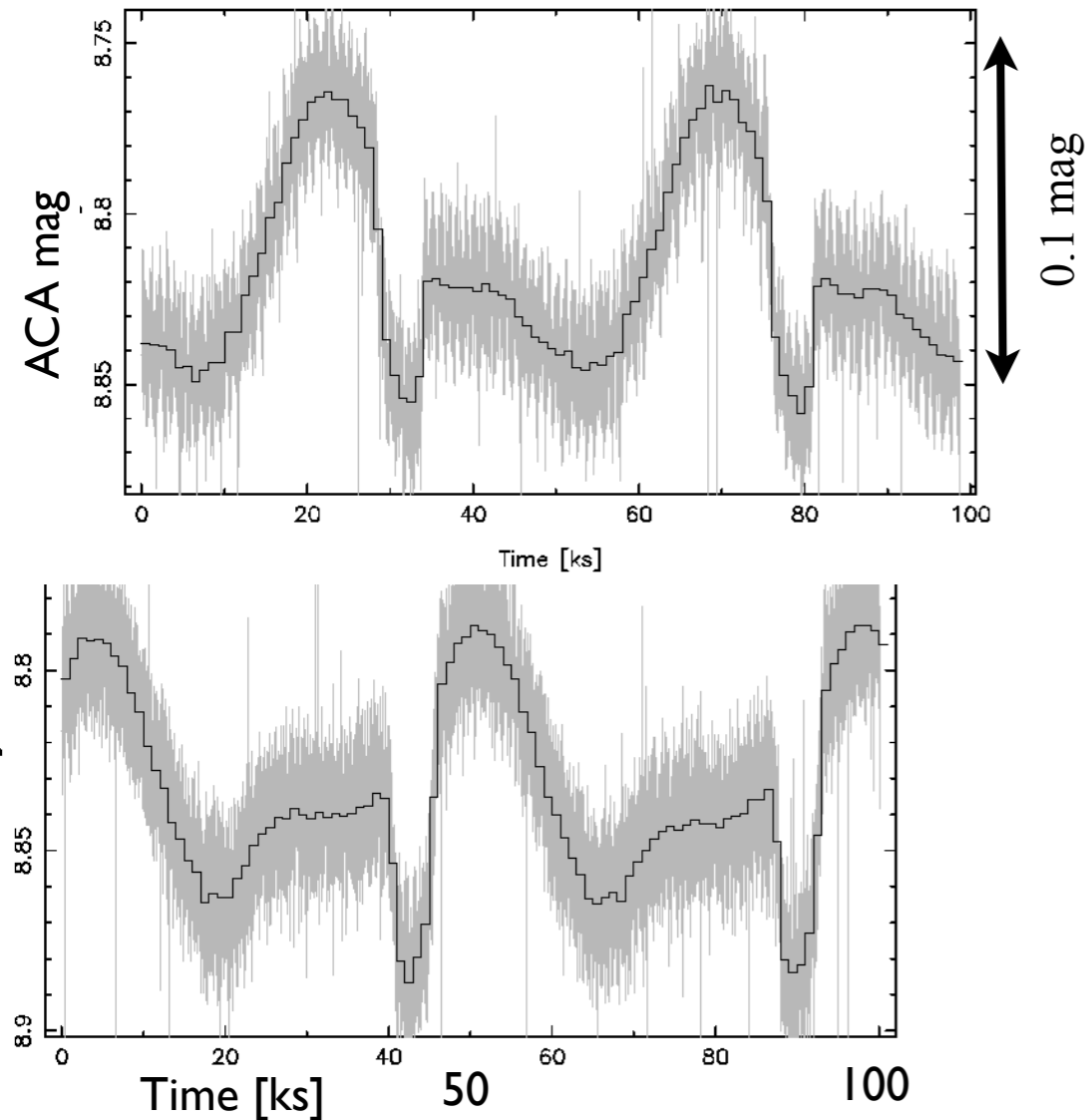
Chandra Optical Light Curves
