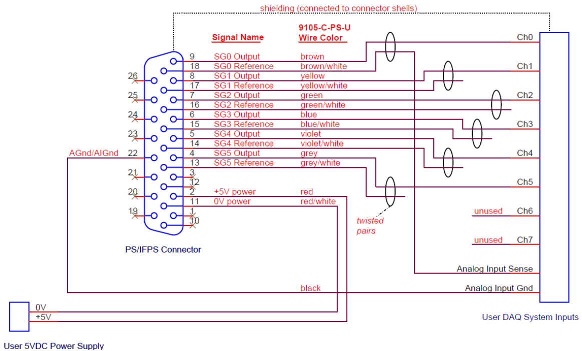
Figure 6.2—Single-Ended Connections to a Data Acquisition System
