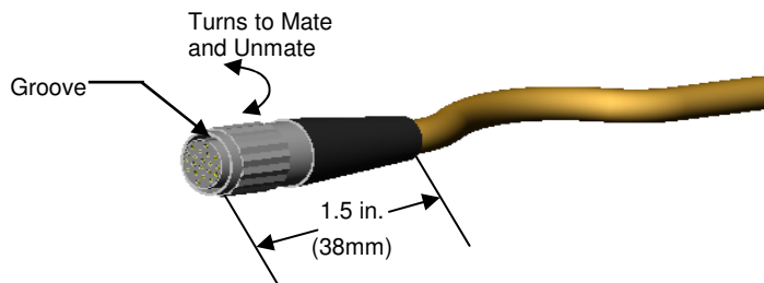
Figure 2.4—Transducer Connector
