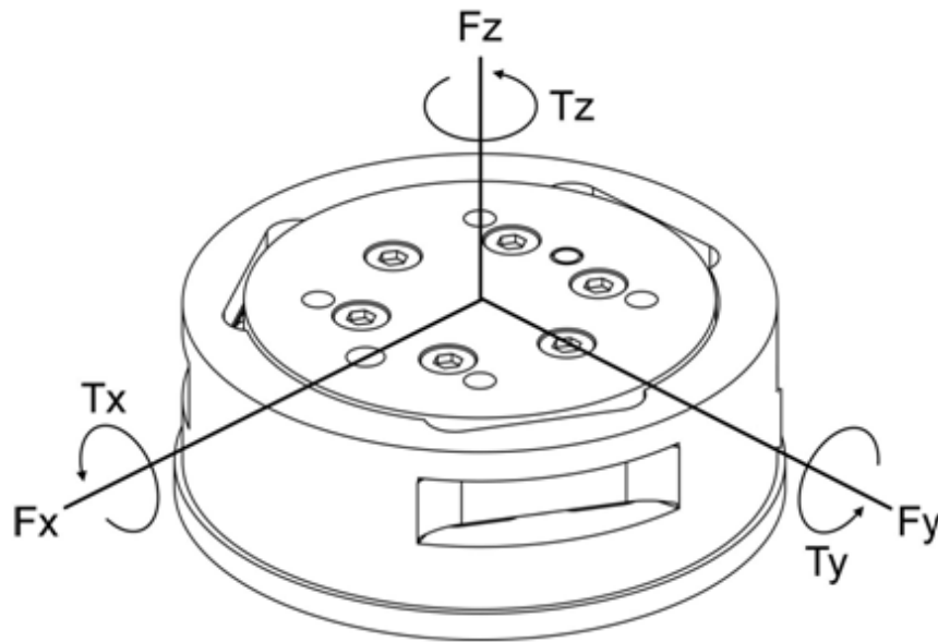
Figure 4.1—Applied Force and Torque Vector on Transducer
