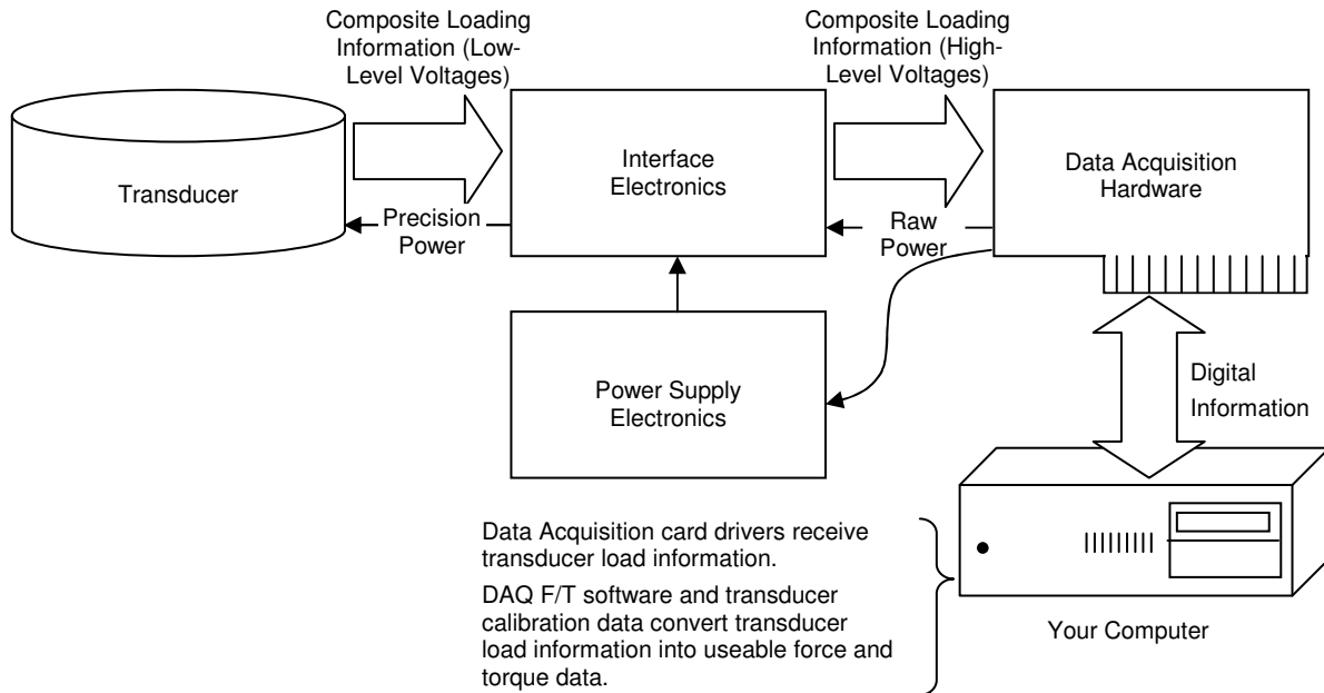
Figure 4.2—Electronic Hardware Outline
