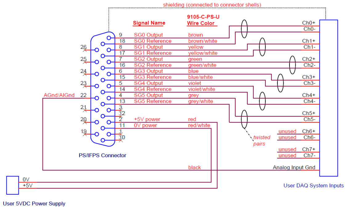
Figure 6.1—Differential Connections to a Data Acquisition System
