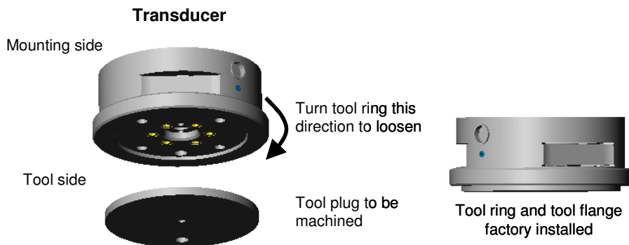
Figure 2.3—Using the tool ring-plug adapter
