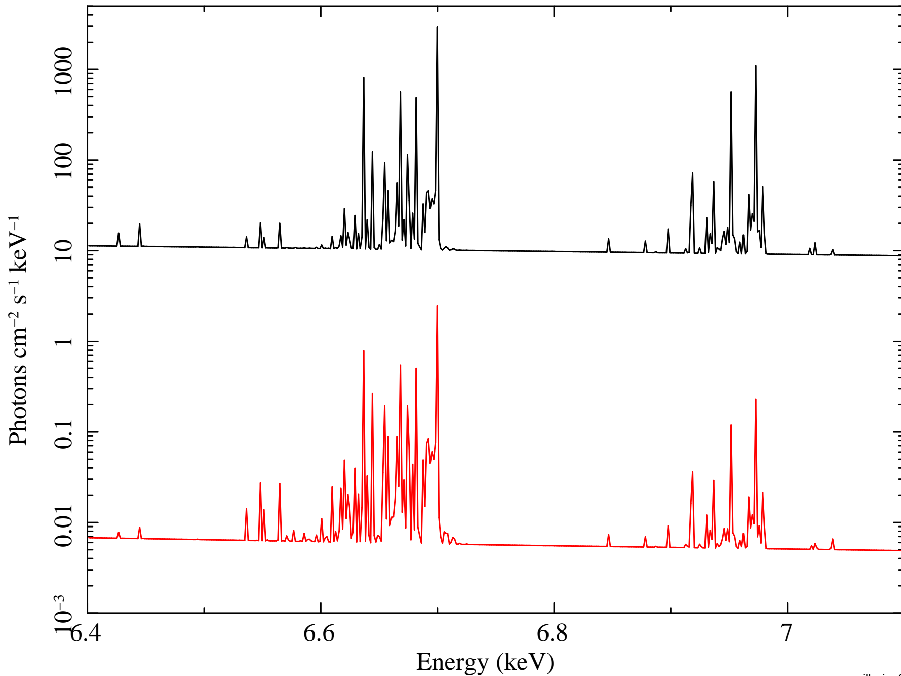
APEC models at Fe XXV K triplet; 4 keV (red) and 7 keV (black)
