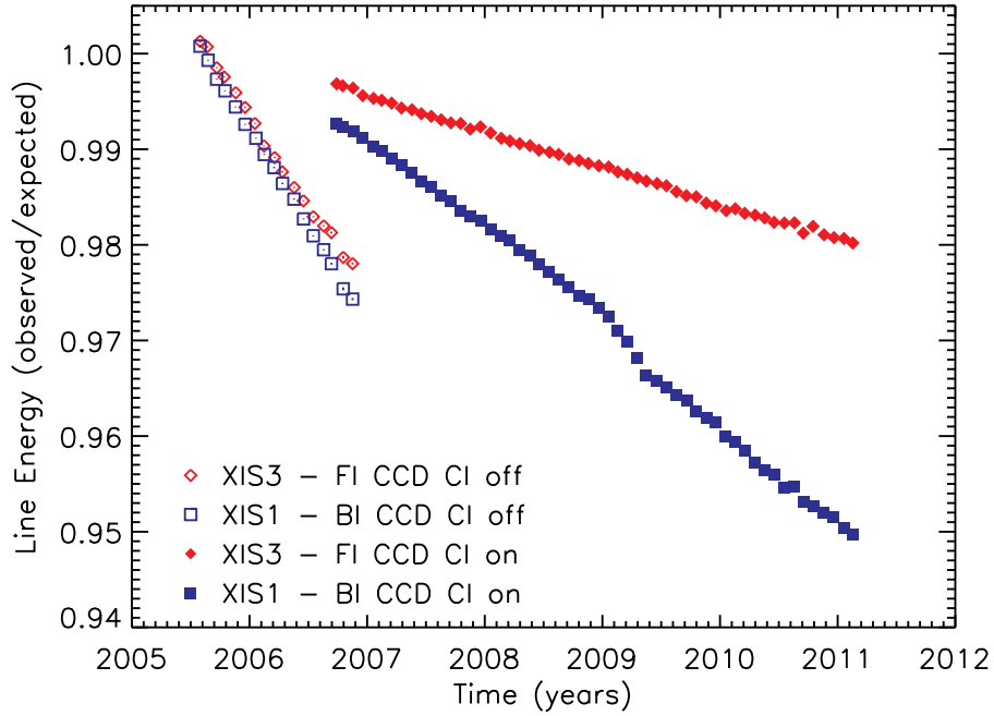
Fig. 6. Fractional change in the XIS line energy over the course of the Suzaku mission, as measured at Mn K\alpha . Different symbols show FI and BI devices with charge injection (CI) on and off. The 1-\sigma error bars are shown but are much smaller than the symbol sizes.
