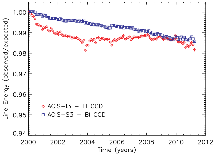
Fig. 7. Fractional change in ACIS line energy over the course of the Chandra mission, as measured at Mn K\alpha . The effects of varying particle background and sacrificial charge are seen in the ACIS-I3 (FI) data. The 1-\sigma error bars are shown but are often smaller than the symbol sizes.
