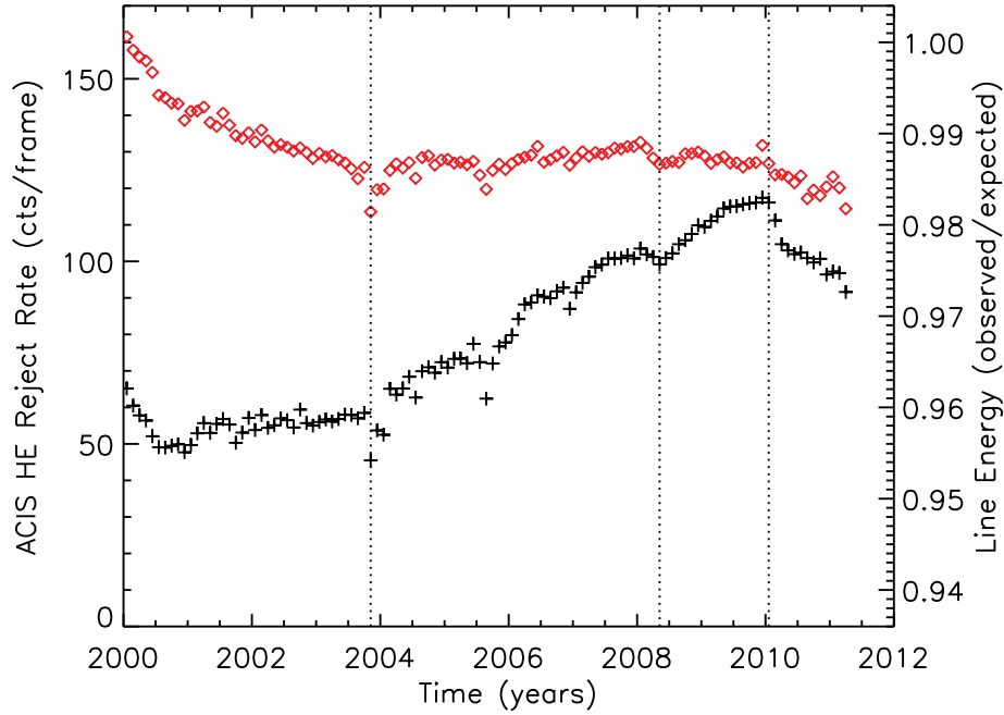
Fig. 8. Time history of the particle background of the Chandra mission, measured as the rate of high energy events on ACIS-S3 (BI), shown as black crosses. The time period and binning are the same as the CTI evolution data. The structure from the varying particle background can be seen in the ACIS FI CCD line energy data, shown in red. The vertical lines demonstrate the simultaneous nature of the structures.
