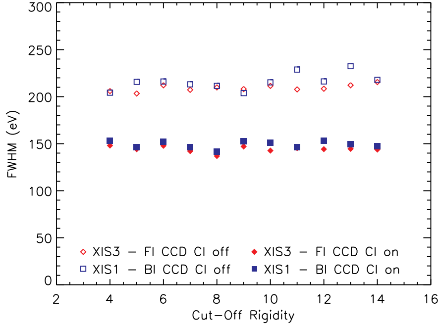
Fig. 13. XIS Mn K\alpha line width (FWHM) as a function of COR, averaging over October–November 2006. Symbols are the same as in Figure 8. Lower cut-off rigidity indicates a higher particle background, therefore the narrower line widths at low COR in the absence of charge injection (open points) are due to sacrificial charge. Use of charge injection overwhelms the effects of sacrificial charge, so no dependence on COR is seen in those data (solid points).
