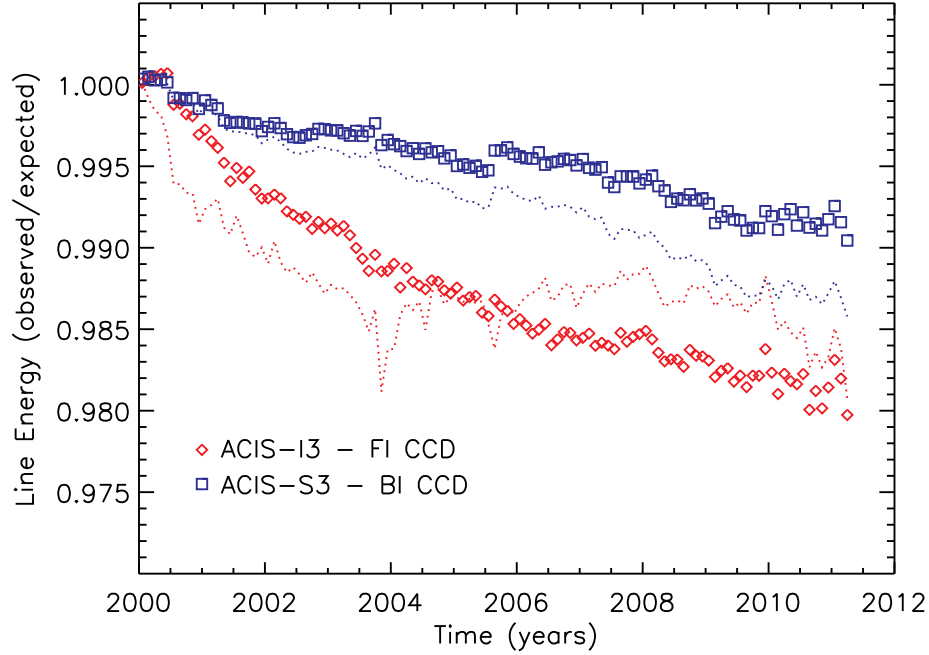
Fig. 11. Fractional change in ACIS line central energy over the course of the Chandra mission, after correcting for sacrificial charge from the particle background. For comparison, the dotted lines show the uncorrected line energy as in Figure 6.
