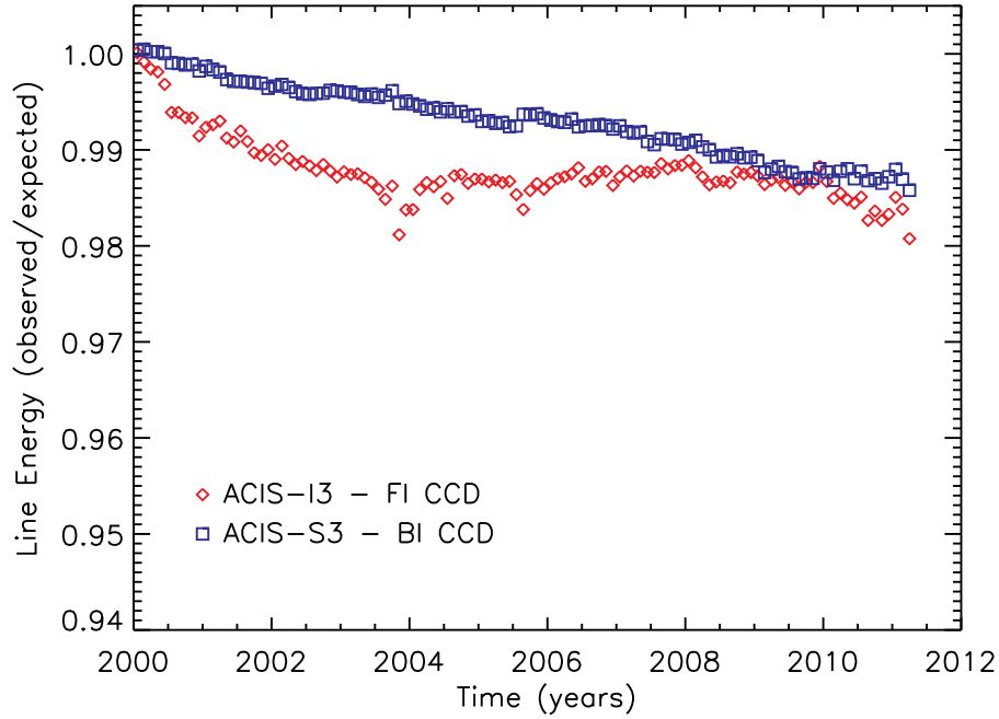
Fig. 6. Fractional change in ACIS line central energy over the course of the Chandra mission, as measured at Mn K\alpha . The effects of varying particle background and sacrificial charge are seen in the ACIS-I3 (FI) data. The 1\text{-}\sigma error bars are not shown but are smaller than the symbol sizes.
