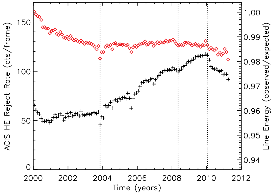
Fig. 7. Time history of the particle background of the Chandra mission, measured as the rate of high energy events on ACIS-S3 (BI). The time period and binning are the same as the CTI evolution data. The structure from the varying particle background can be seen in the ACIS FI CCD line energy data, shown in red. The vertical lines demonstrate the simultaneous nature of the structures.
