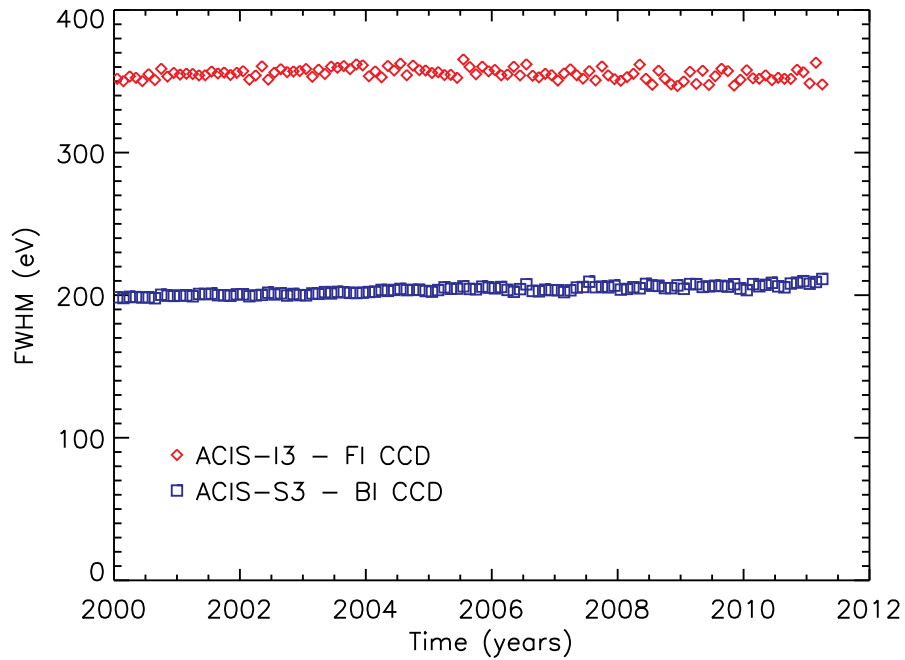
Fig. 9. Change in ACIS line width over the course of the Chandra mission, as measured at Mn K\alpha . The 1-\sigma error bars are not shown but are smaller than the symbol sizes.
