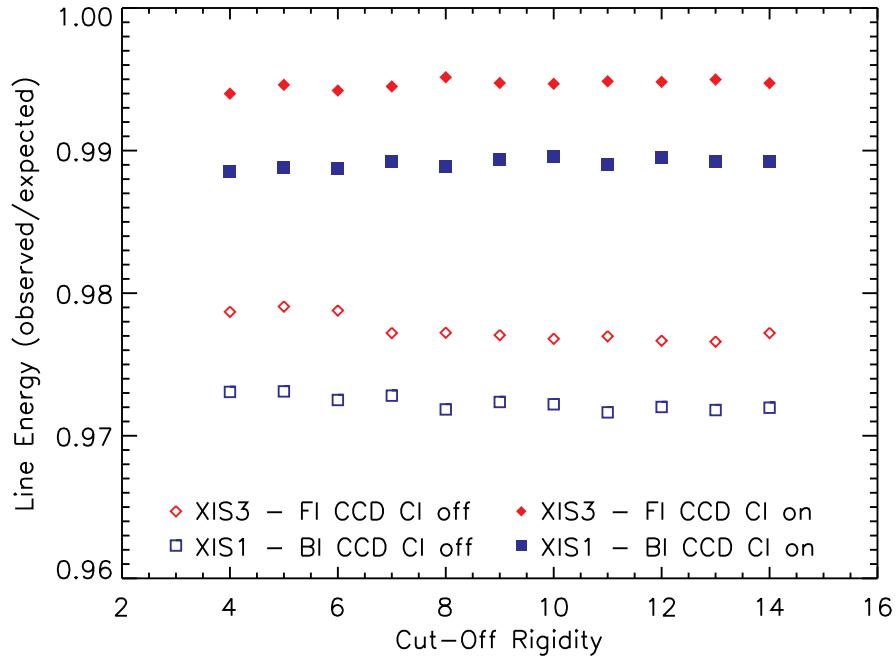
Fig. 12. Fractional change in the XIS line energy as a function of geomagnetic cut-off rigidity (COR), averaging over October-November 2006. Symbols are the same as in Figure 5. Without charge injection, there is a weak dependence of line energy with COR, with higher line energy associated with lower COR, as is expected for sacrificial charge. The use of charge injection overwhelms the effects of sacrificial charge (solid points) from the particle background. The 1\text{-}\sigma error bars are not shown but are smaller than the symbol sizes.
