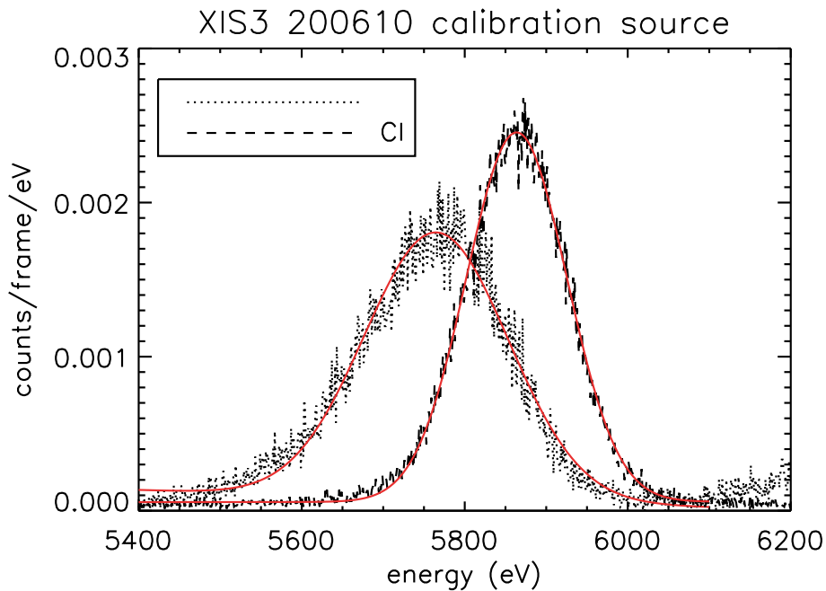
Fig. 3. Spectrum of the Mn K\alpha line at 5.9 keV for the XIS FI CCD. Without charge injection (dotted line), the line is broader and shifted to lower energies. Charge injection (dashed line) improves both the line centroid and the width. The red line is the best fit Gaussian plus linear background.
