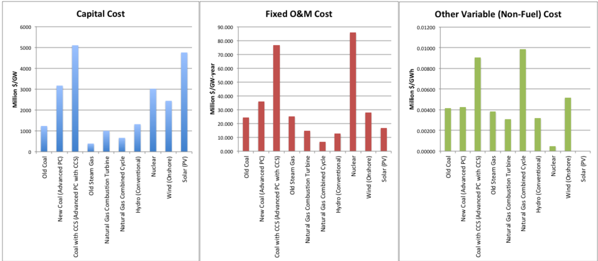
Figure 2-9 Capital costs (a), fixed operation and maintenance costs (b), and variable costs (c) for various electricity generation technologies (Data Sources: Short et al., 2009; EIA, 2010b).
