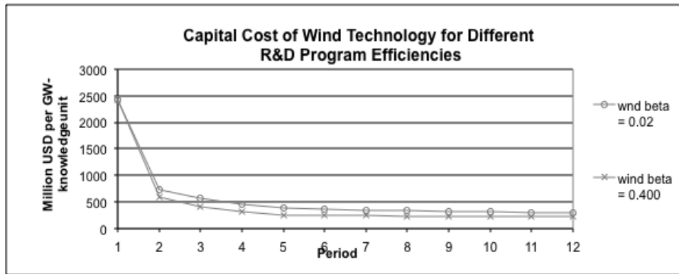
Figure 5-17 Comparison of capital cost trajectories with low (o) and high (x) WIND R&D investment efficiency under a MODERATE (50% BAU) carbon target
