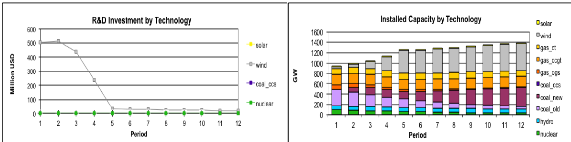
Figure 5-5 Optimal R&D investments (left) and installed capacities (right) for various learning scenarios under BAU
