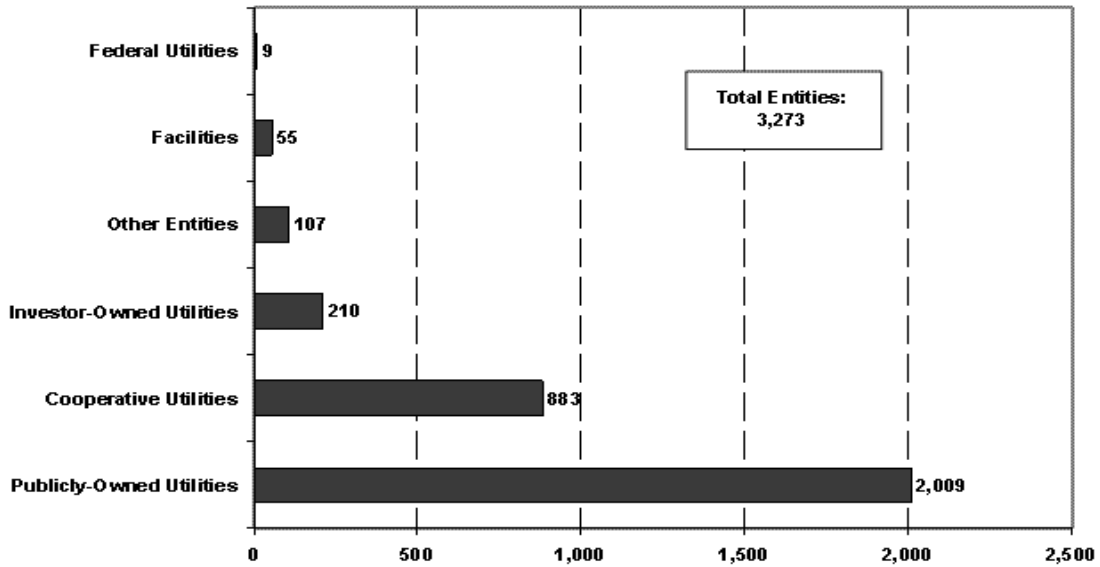
Figure 2-7 Composition of U.S. Electric Utilities 2007 (EIA, 2007a)
