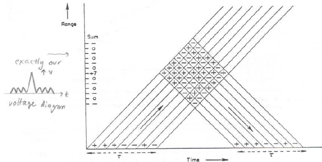
FIG. 9. Range-time diagram for a Barker-coded pulse, which is split into seven elements with + or - phases, as shown. The contributions of the 49 cells are obtained by multiplication, as shown. Only at the central range do these consistently add up to give a sum of +7 contributions. At the other ranges the sums are zero or -1, so nearly all the signal comes from the central range.
