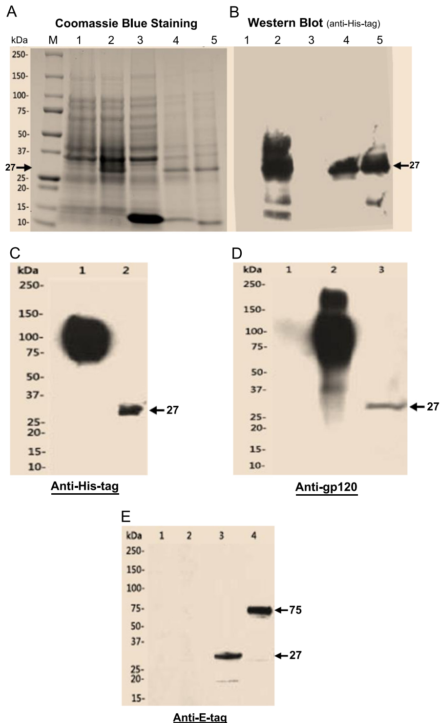
Fig. 2. Expression and purification of the designed single-chain antibody VRC01 in E. coli . (A) Polyacrylamide gel with Coomassie blue staining. Lane 1, cell pellet total proteins of un-induced; 2, cell pellet total proteins of induced; 3, supernatant of cell lysate; 4, pellet of cell lysate; 5, Urea-solubilized inclusion bodies. (B) Western blot of the same purified protein samples from A using anti-His-tag antibody. The specific band (~27 kDa) of scFv antibody VRC01 is indicated by the arrow in (A and B). Western blot to verify the purified single-chain antibody VRC01. (C) Western blot with anti-His-tag antibody. Lane 1, gp120, 2, scFv_VRC01. (D) Far-Western blot first with the binding of bait protein gp120, then with the anti-gp120 antibody. Lane 1, BSA; 2, gp120, 3, scFv-VRC01. (E) Western blot of scFv-VRC01 and scFv-VRC01- \beta -domain fusion protein (~75 kDa). Both of the samples are labeled as follows: Lane 1, Supernatant of strain containing plasmid scFv-VRC01; 2, Supernatant of strain containing plasmid scFv-VRC01- \beta -domain; 3, Cell pellet of strain containing plasmid scFv-VRC01; 4, Cell pellet of strain containing plasmid scFv-VRC01- \beta -domain.
