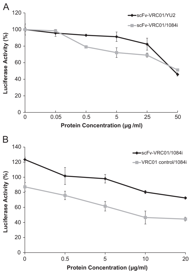
Fig. 3. Functional analysis of purified single-chain antibody VRC01. (A) Neutralization assay of the scFv-VRC-1 against different strains of HIV-1: YU2 (subtype B), 1084i (subtype C). (B) Comparison of the scFv VRC01 antibody and corresponding VRC01 IgG antibody.
