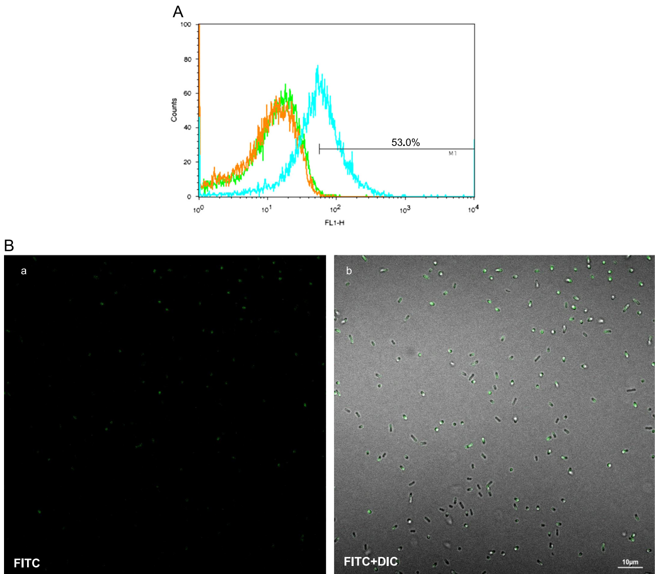
Fig. 4. Identification of Surface display of fusion protein on E. coli . (A) Bacterial sample cells ( E. coli ) were treated with FITC-conjugated anti-rabbit IgG antibody and analyzed by Flow cytometer. Orange, unstained bacterial cells as negative control; green, stained bacteria cells harboring the vector only; cyan, stained bacteria harboring the scFv-VRC01- \beta -domain plasmid. The total gated positive cell percentage (M1) is shown in the figure. (B) Bacterial Cells displaying scFv-VRC01 on the surface using confocal microscopy. The positive stained bacterial cells by FITC-conjugated anti-rabbit IgG antibody are shown in green. The same image is shown in (a) dark background window (FITC). (b) the bright background window (FITC)+(DIC) (differential interference contrast). The size bar showing in the picture is 5.0 \mu m in (a) and 10.0 \mu m in (b).
